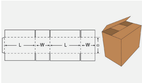
R.S.C. (Regular Slotted Container)
