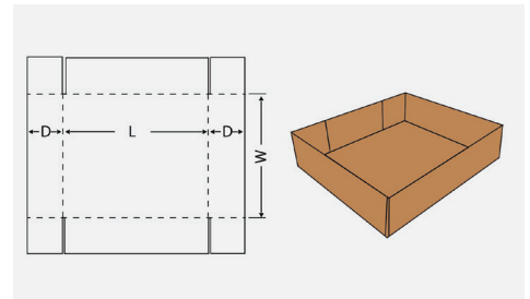
Telescope Tray (Side Slotted Tray)
