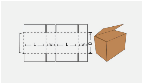
F.O.L. (Full Over Lap)
